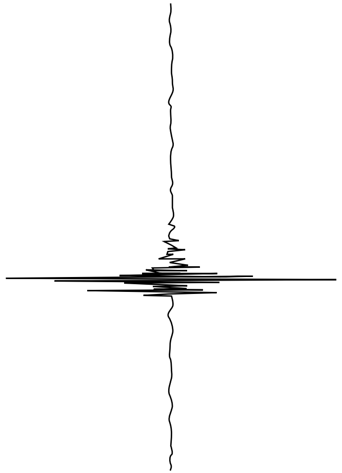
BGS seismograph trace 26 XII 2006 page 1
